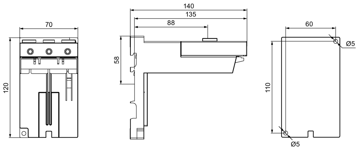
Figure C-55 3RU2946-3AA01
