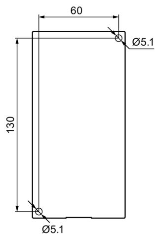
Figure C-46 Drilling diagram for 3RT2.4. contactors (size S3)
