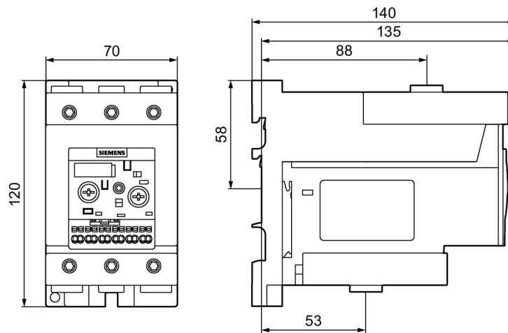
Figure C-37 3RB3.4.-..D0 and 3RU2946-3AA01
