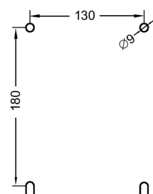
Figure C-49 Drilling diagram for 3RT1.7. contactors (size S12)
