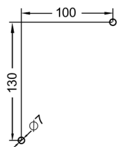
Figure C-47 Drilling diagram for 3RT1.5. contactors (size S6)
