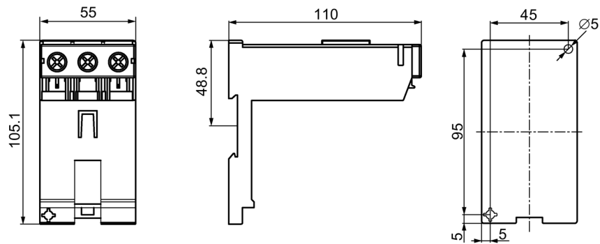
Figure C-54 3RU2936-3AA01
