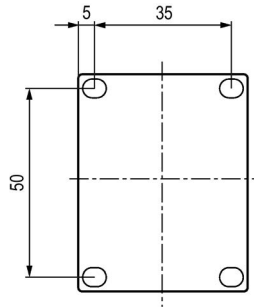
Figure C-42 Drilling plan for contactors with screw-type connections and ring cable lug connections (size S00)
