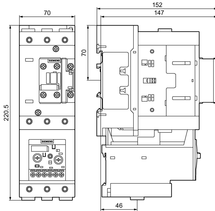
Figure C-34 3RB3.4-...B0
