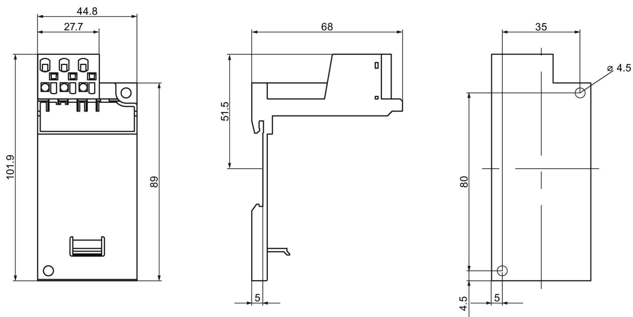
Figure C-51 3RU2916-3AC01
