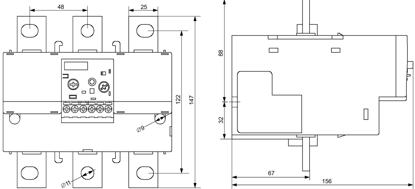
Figure C-19 3RB2.6
