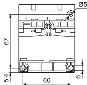
Figure C-41 3RB3.4.-..X. - drilling diagram
