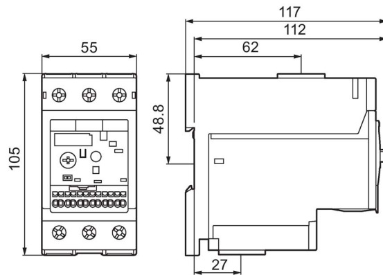
Figure C-31 3RB3.3.-..D0 and 3RU2936-3AA01
