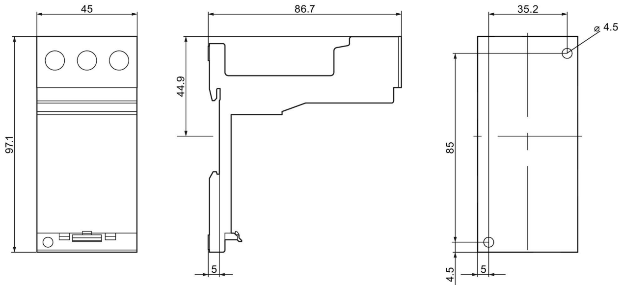
Figure C-52 3RU2926-3AA01
