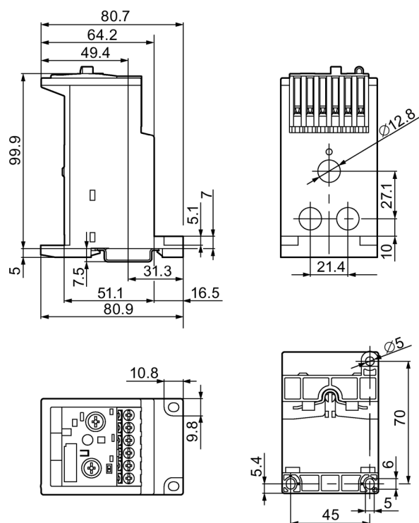
Figure C-32 3RB3.3-..W.
