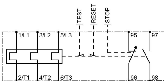
Figure 12-5 Thermal overload relay, S3
