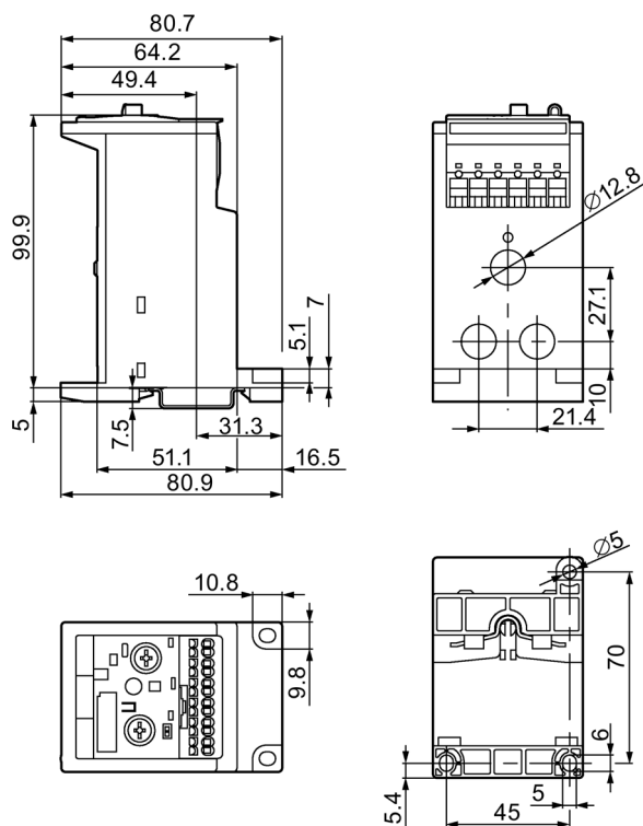
Figure C-33 3RB3.3.-.X.
