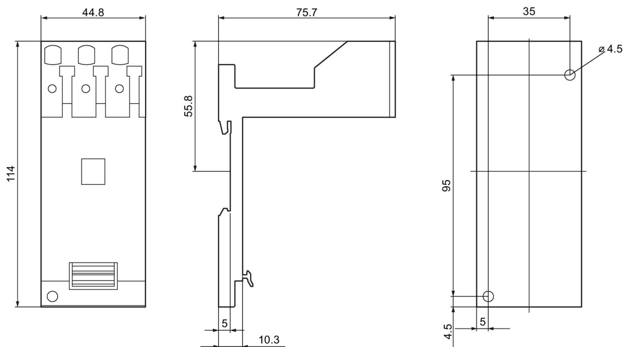
Figure C-53 3RU2926-3AC01
