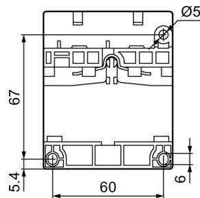
Figure C-39 3RB3.4-..W. - drilling diagram
