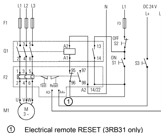
Figure 12-21 3RB3.1-...B0
