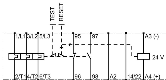
Figure 12-15 3RB31 electronic overload relay, screw-type connection system, S00
