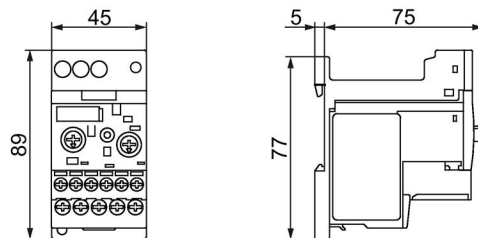
Figure C-21 3RB3.1-...B0 and 3RU2916-3AA01
