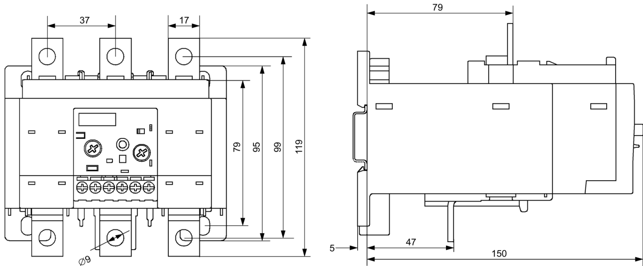
Figure C-17 3RB2.5
