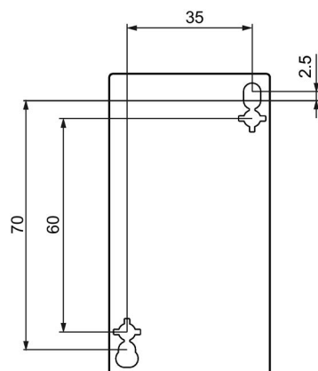
Figure C-44 Drilling plan for 3RT2.2. contactors (size S0)
