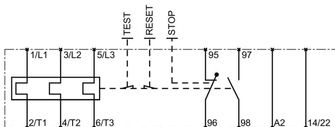
Figure 12-1 Thermal overload relay, screw-type and ring cable lug connection systems, S00
