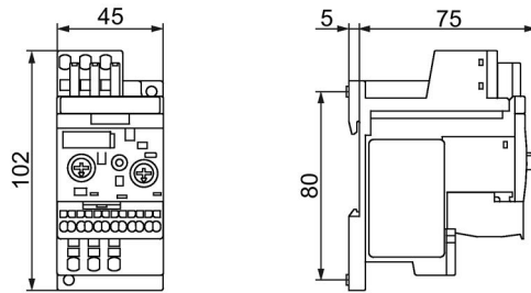
Figure C-23 3RB3.1.-..E0 and 3RU2916-3AC01
