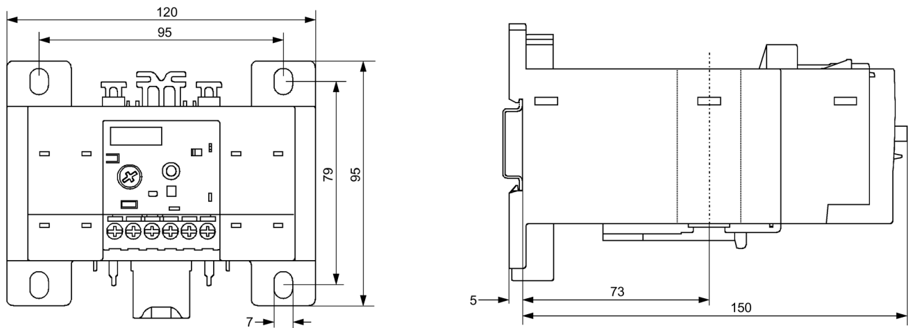
Figure C-18 3RB2.5-..W 3RB2.5-..X
