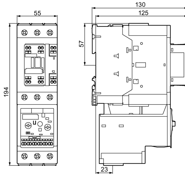
Figure C-30 3RB3.3.-..D0
