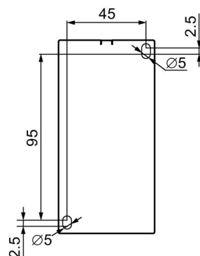
Figure C-45 Drilling plan for 3RT2.3. contactors (size S2)
