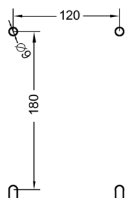
Figure C-48 Drilling diagram for 3RT1.6. contactors (size S10)
