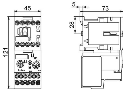
Figure C-20 3RB3.1-...B0
