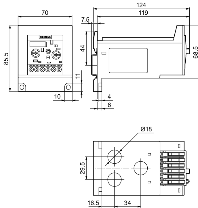
Figure C-38 3RB3.4-..W.
