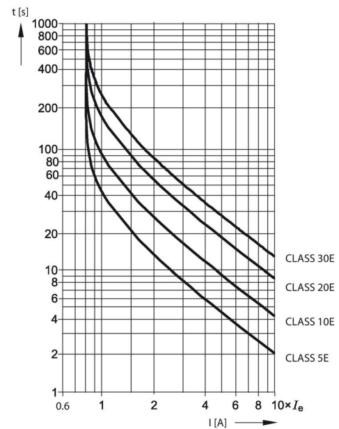
Tripping characteristic 2
