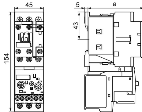
Figure C-24 3RB3.2-..B0
