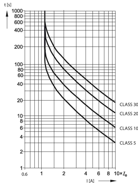
Tripping characteristic 1
