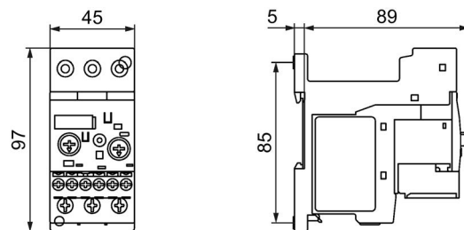
Figure C-25 3RB3.2-..B0 and 3RU2926-3AA01
