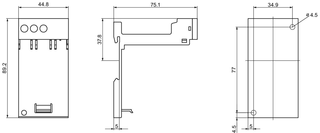
Figure C-50 3RU2916-3AA01
