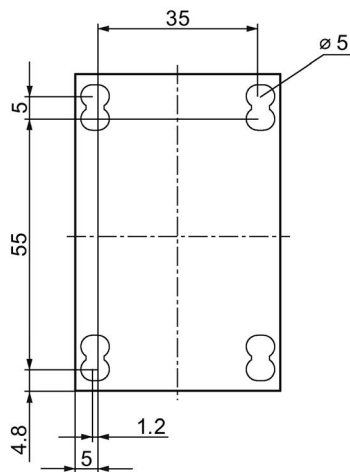
Figure C-43 Drilling plan for contactors with spring-loaded connections (size S00)
