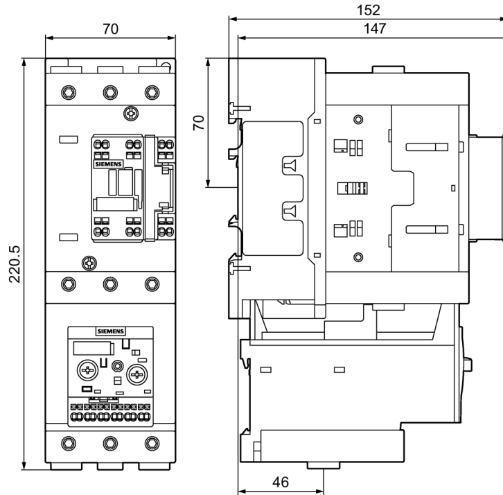
Figure C-36 3RB3.4.-..D0
