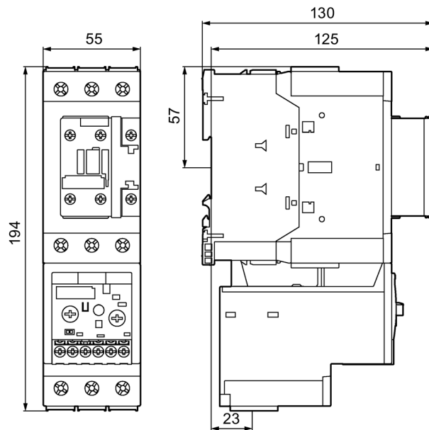
Figure C-28 3RB3.3-..B0
