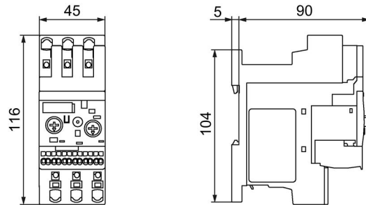
Figure C-27 3RB3.2.-..E0 and 3RU2926-3AC01
