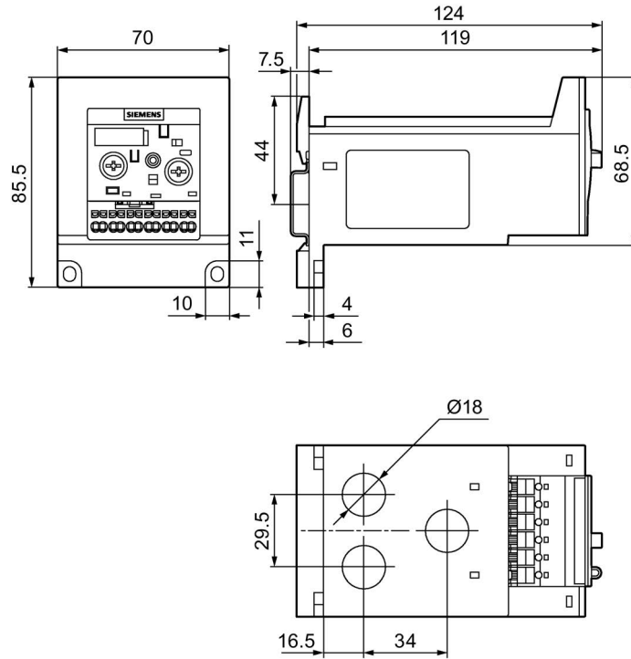
Figure C-40 3RB3.4.-..X.
