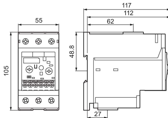
Figure C-29 3RB3.3-..B0 and 3RU2936-3AA01
