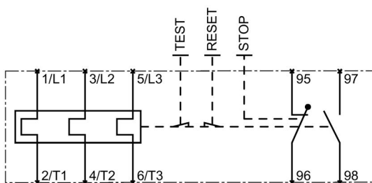
Figure 12-4 Thermal overload relay, S2
