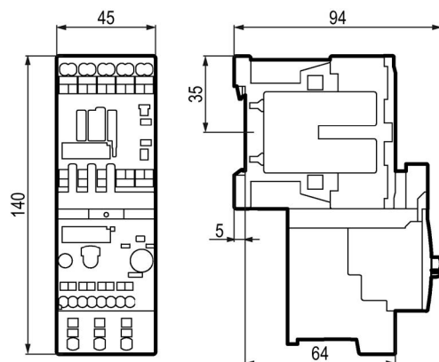
Figure C-3 3RU2116-..C0
