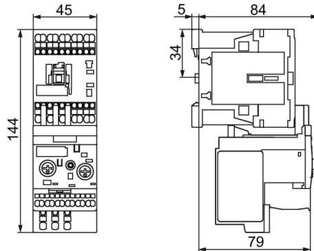
Figure C-22 3RB3.1.-..E0
