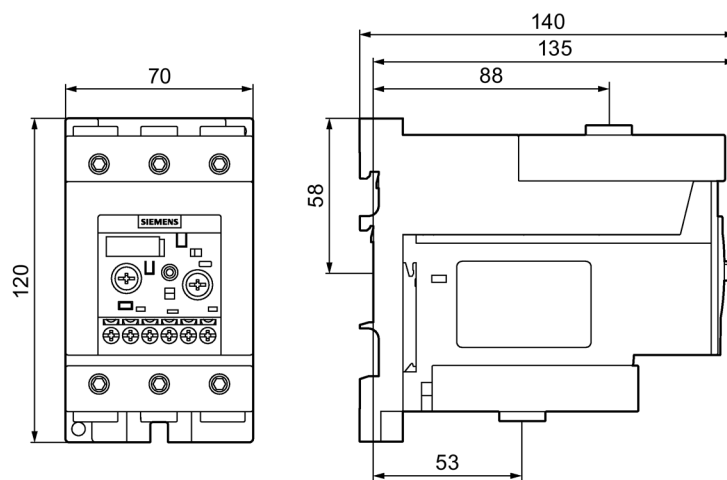
Figure C-35 3RB3.4-...B0 and 3RU2946-3AA01
